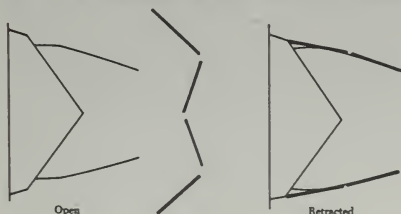
FIGURE 2-38. Mechanical blockage thrust reverser.
